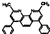
Structural formula 2:
